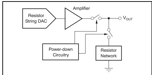
Figure 113. Output Stage During Power-Down
